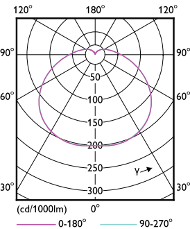
Light Distribution Diagram - TForce Core HB 3Klm 30W E27 865 WV
