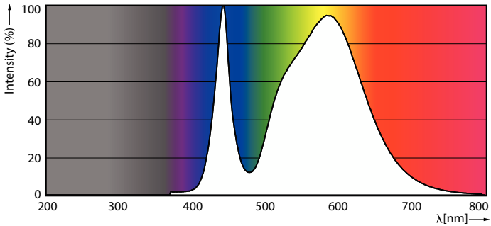
Spectral Power Distribution Colour - Ecofit E Mains 1200mm 16W 740 T8
