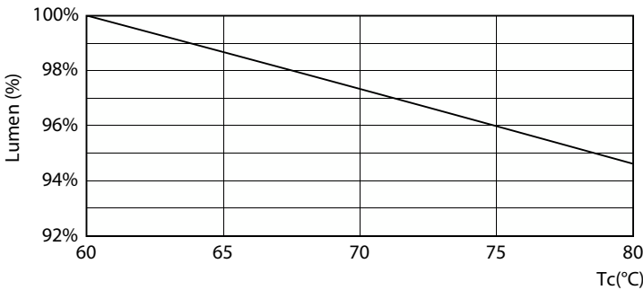
Lumen Maintenance Diagram - Ecofit E Mains 1200mm 16W 740 T8
