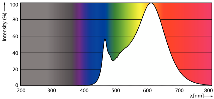
Spectral Power Distribution Colour - CorePro LEDtube 1200mm 16W830 G5 I MX
