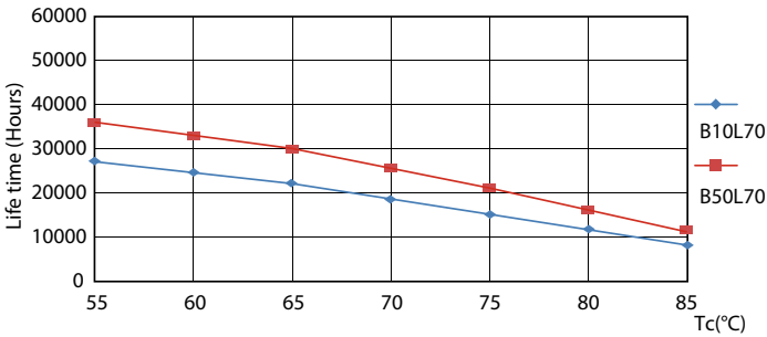
Life Expectancy Diagram - CorePro LEDtube 1200mm 16W830 G5 I MX
