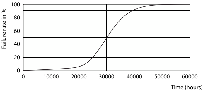
Life Expectancy Diagram - CorePro LEDtube 600mm 8W830 G5 I MX
