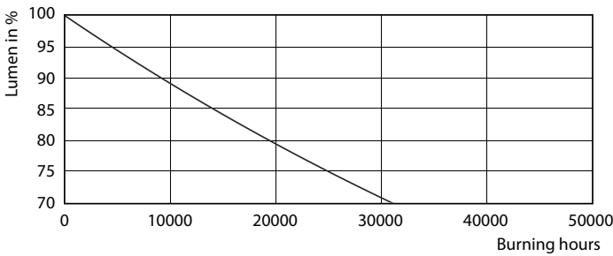
Lumen Maintenance Diagram - CorePro LEDtube 600mm 8W830 G5 I MX
