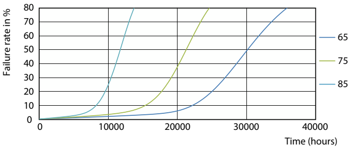
Life Expectancy Diagram - CorePro LEDtube 600mm 8W830 G5 I MX
