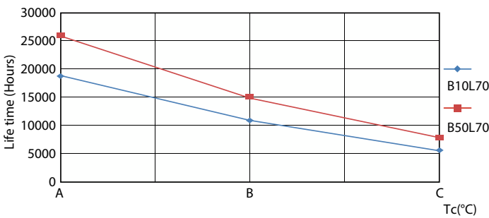
Life Expectancy Diagram - Ecofit Mains LEDtube 1200mm 16W 740 G
