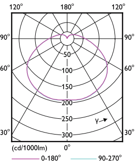
Light Distribution Diagram – TForce Core HB 5Klm 50W E40 865 WV
