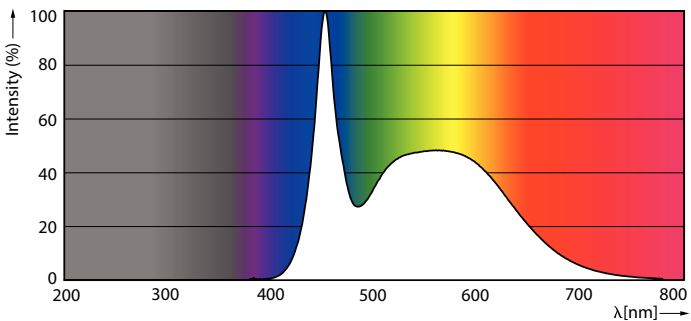
Spectral Power Distribution Colour – TForce Core HB 5Klm 50W E40 865 WV
