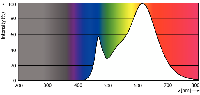
Spectral Power Distribution Colour - EcoHome LEDBulb 14W E27 3000KHV 1PF/20AR
