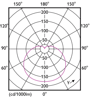
Light Distribution Diagram - EcoHome LEDBulb 14W E27 3000KHV 1PF/20AR
