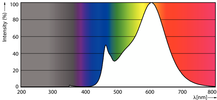
Spectral Power Distribution Colour - LEDClassic 6W G120 E27 830 CLND1PF/6
