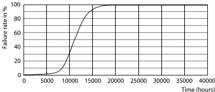
Life Expectancy Diagram - LEDClassic 6W G120 E27 830 CLND1PF/6
