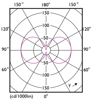
Light Distribution Diagram - LEDClassic 6W G120 E27 830 CLND1PF/6
