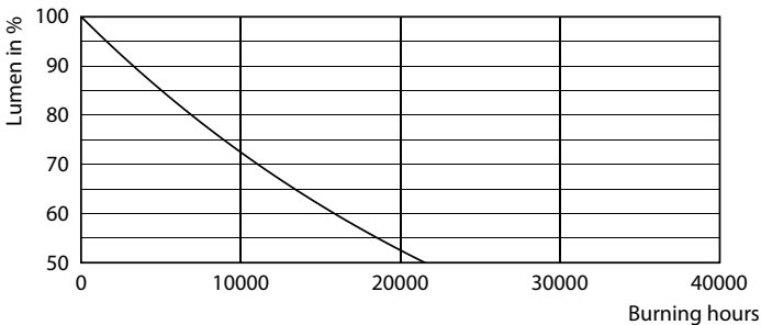
Lumen Maintenance Diagram - LEDClassic 6W G120 E27 830 CLND1PF/6
