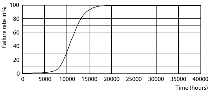
Life Expectancy Diagram - LEDClassic 6W A60 E27 830 CLND1PF/10
