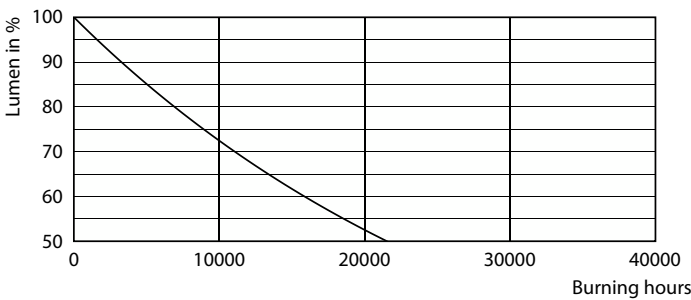
Lumen Maintenance Diagram - LEDClassic 6W A60 E27 830 CLND1PF/10
