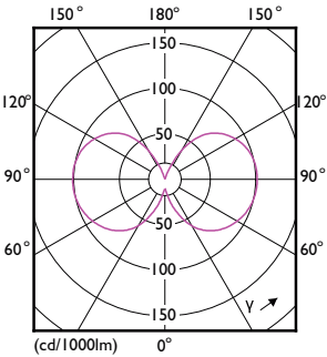
Light Distribution Diagram - LEDClassic 6W A60 E27 830 CLND1PF/10
