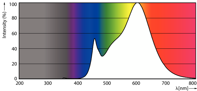
Spectral Power Distribution Colour - LEDClassic 6W A60 E27 830 CLND1PF/10
