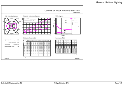
Classic LEDGlobe ND 6-60W G93 E27 827 CL
