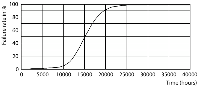
Life Expectancy Diagram - LED classic 5.5W ST64 E27GOLD SP D 1PF/6
