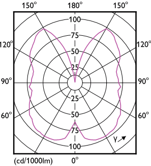
Light Distribution Diagram - LED classic 5.5W ST64 E27GOLD SP D 1PF/6
