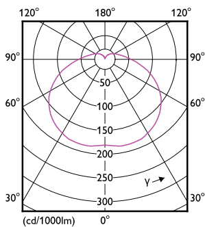
Light Distribution Diagram - LEDBright 20W E27 3000K HV 1PF/12 AR
