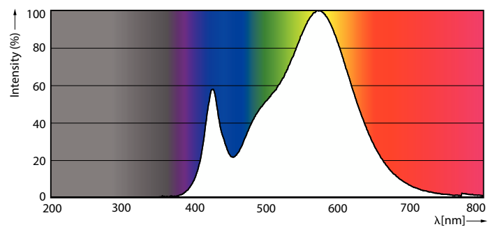
Spectral Power Distribution Colour - LEDBright 20W E27 3000K HV 1PF/12 AR
