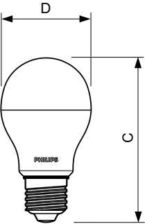
Bulb A55 220-250V 9-80W 950lm 6500K E27
