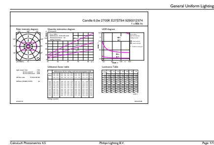
CorePro LEDbulb ND 6-60W ST64 827
