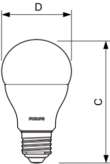
LED 9.5-60W E27 830
