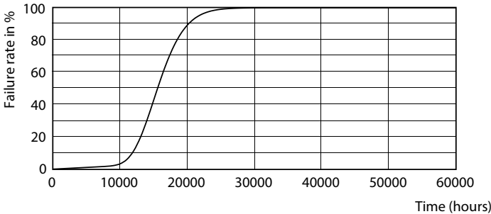
LEDspot ESS 50W GU10 PAR16 840 36D ND
