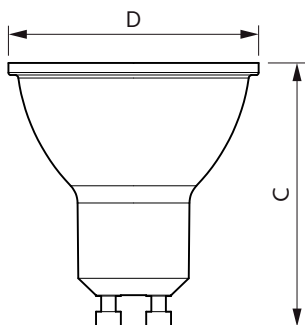
GU10 230V 5.5W-50W 345lm 36D 2700K ND
