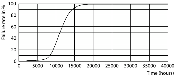
Life Expectancy Diagram - EcoHome LEDBulb 4W E27 6500K G45 1PF AR
