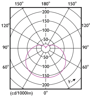
Light Distribution Diagram - EcoHome LEDBulb 4W E27 6500K G45 1PF AR
