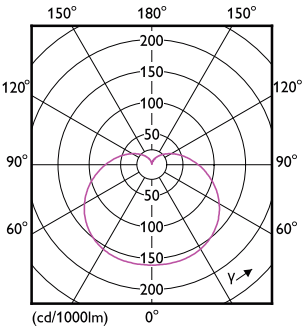
Light Distribution Diagram - EcoHome LEDBulb 4W E27 3000K G45 1PF AR
