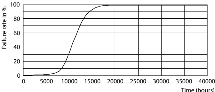
Life Expectancy Diagram - EcoHome LEDBulb 4W E27 3000K G45 1PF AR
