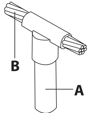
Ground Rod To Wire Connections
