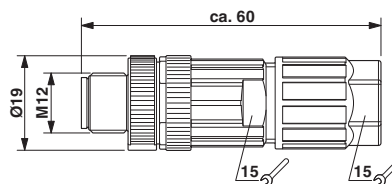
Conector macho SPEEDCON M12, recto
