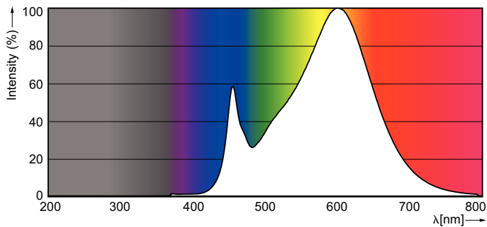
LEDtube, MASTER LEDtube 1200mm HO 16W /830 T8 RN
