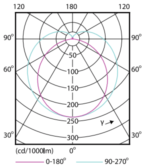
LEDtube, MASTER LEDtube 1200mm HO 16W /830 T8 RN
