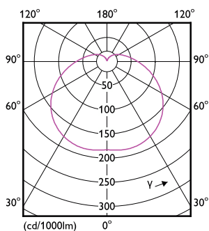
Light Distribution Diagram - TForce Core HB 40W E27 865 WV G3
