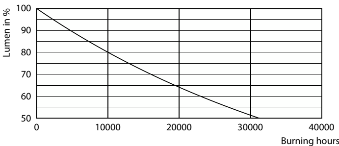
Lumen Maintenance Diagram - TForce Core HB 40W E27 865 WV G3
