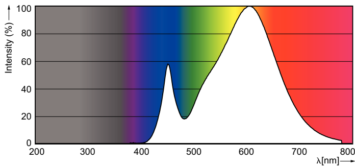
CorePro LEDspotMV D 5.7-60W R63
