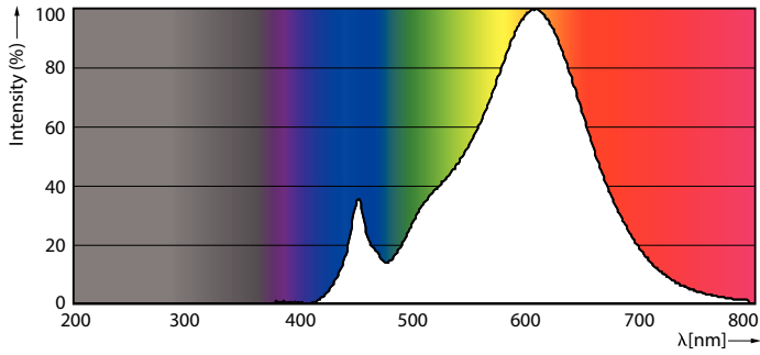
LEDcapsule_1,6W_G9_827
