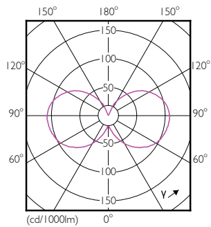
Light Distribution Diagram - LEDcapsule 25W G9 827 100-240 ND
