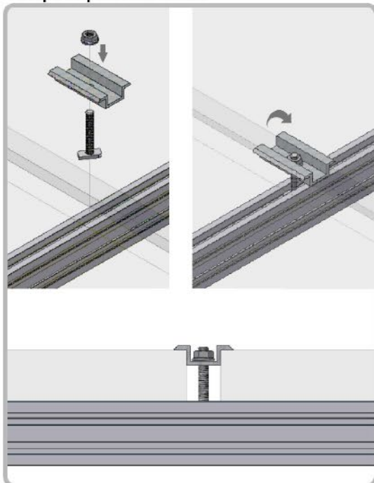
Grapa de panel intermedia
