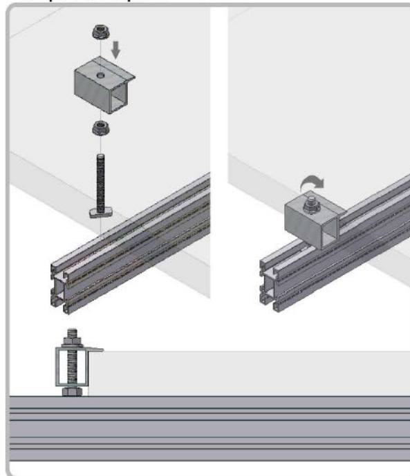
Grapa final de panel
