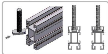
Grapa de panel intermedia
